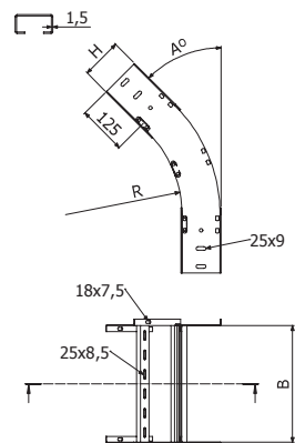
H75-H120
